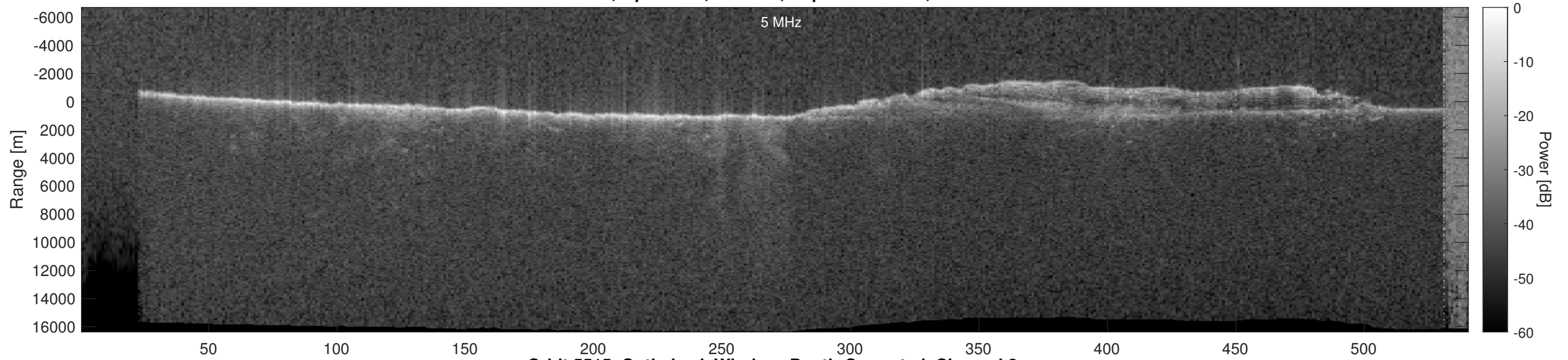
Orbit 5515, Optimized, Window, Depth-Corrected, Channel 2
