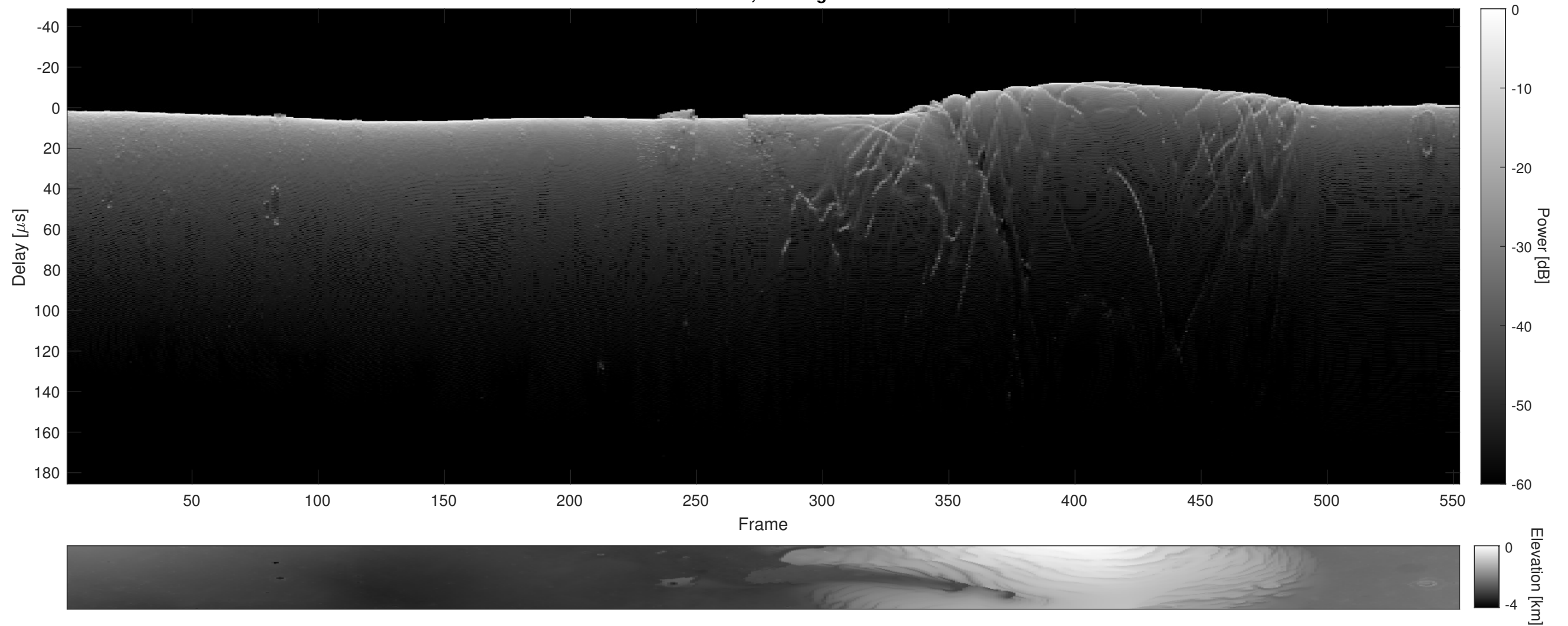
Orbit 5518, Cluttergram
