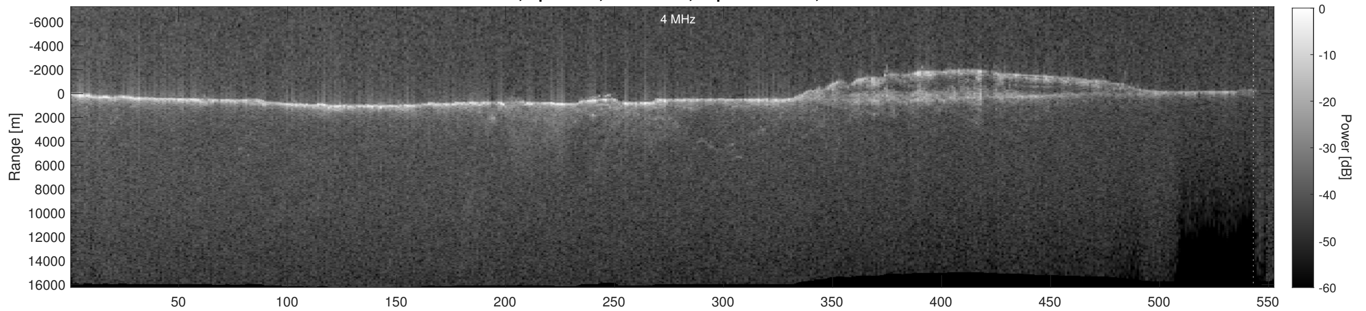
Orbit 5518, Depth-Corrected Cluttergram
