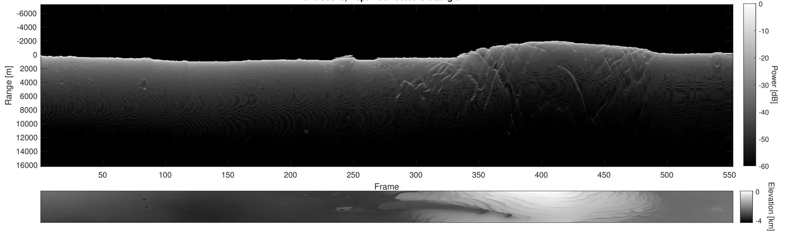
Orbit 5518, Depth-Corrected Cluttergram
