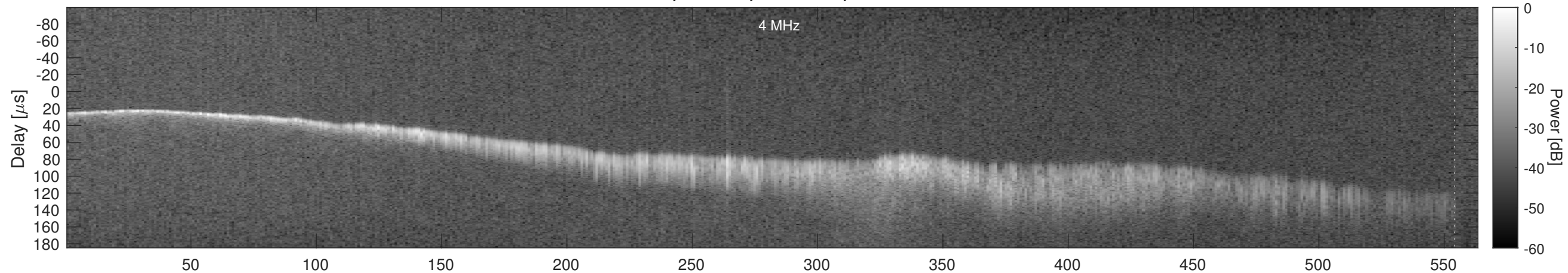
Orbit 5527, Window, Channel 2, Chapman
