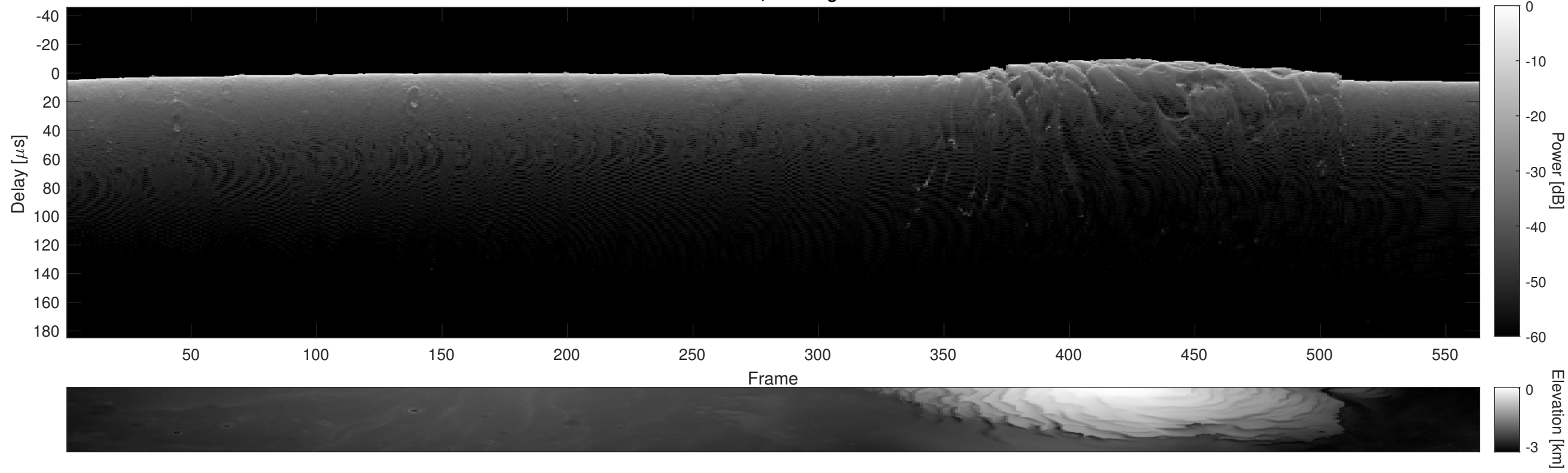
Orbit 5527, Cluttergram
