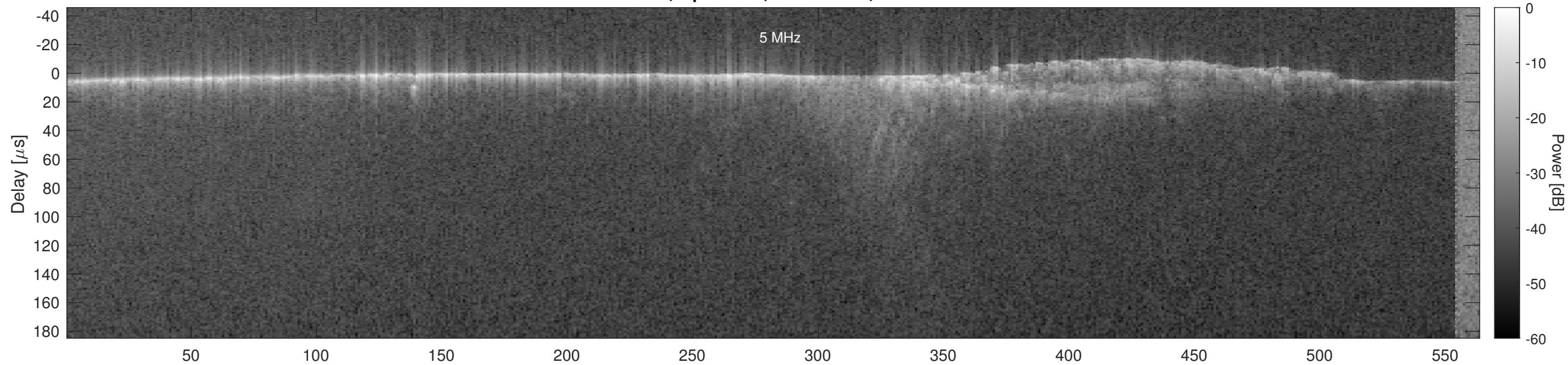
Orbit 5527, Optimized, No Window, Channel 2
