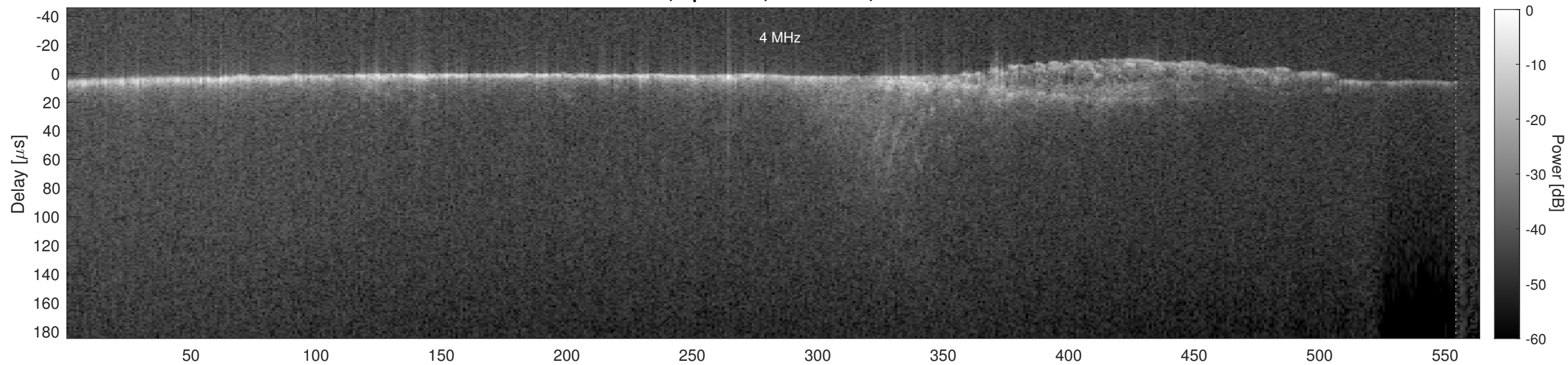
Orbit 5527, Cluttergram
