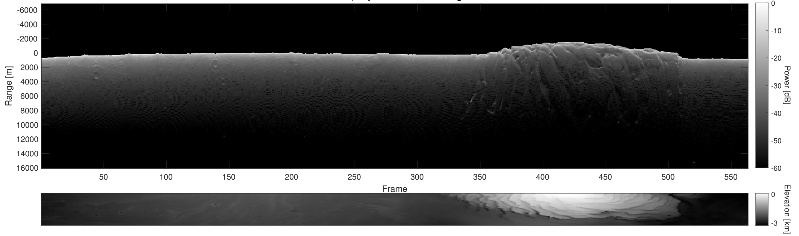
Orbit 5527, Depth-Corrected Cluttergram
