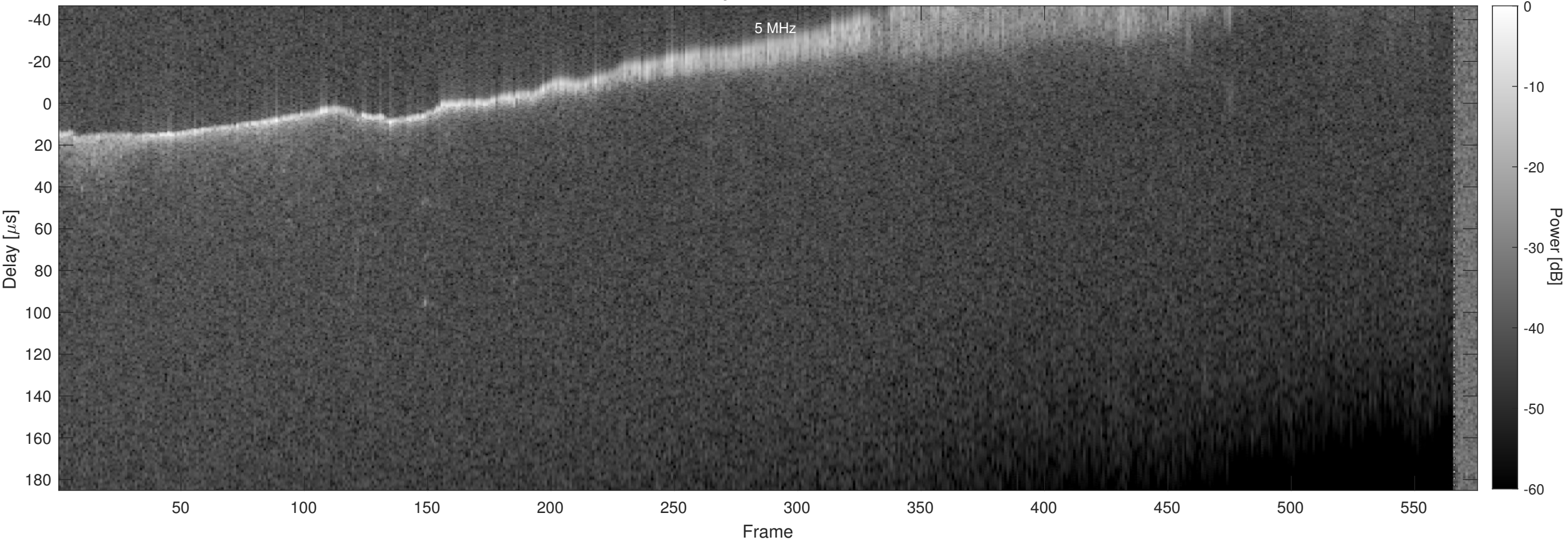
Orbit 5535, Chapman, Window, Channel 2
