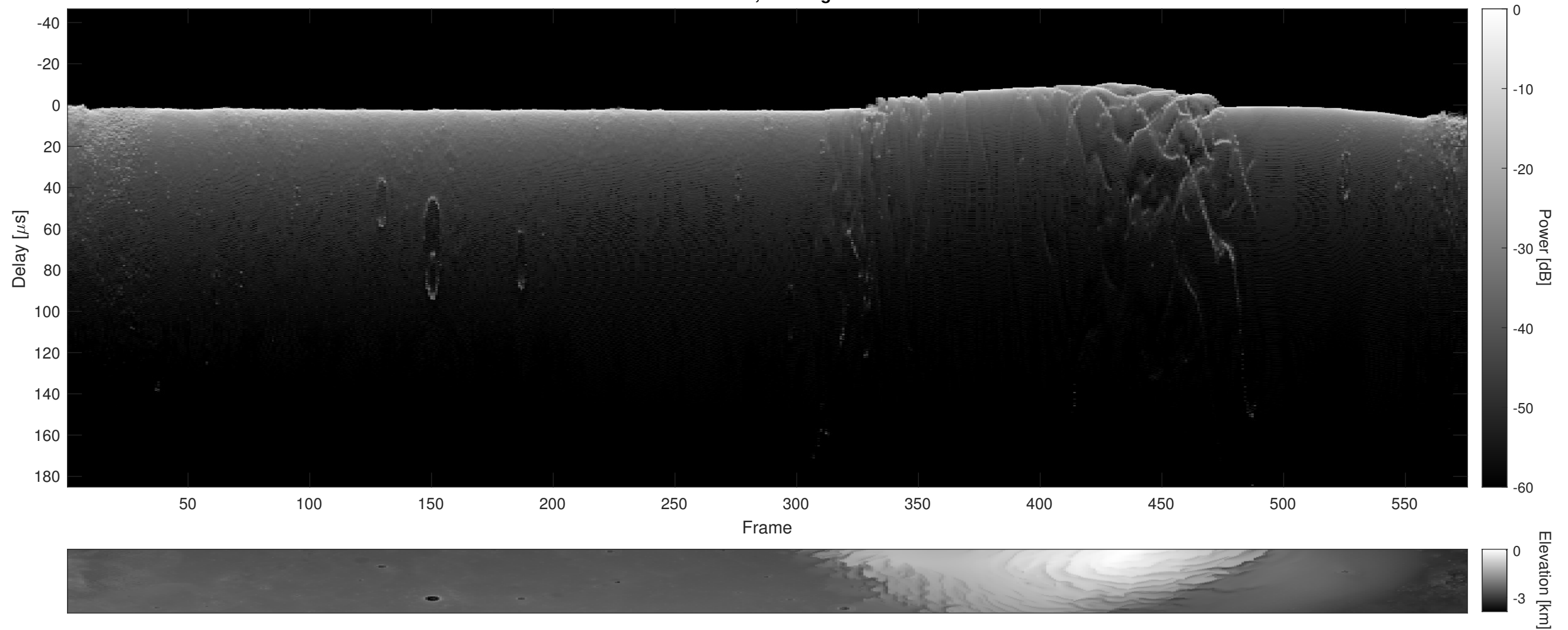
Orbit 5535, Cluttergram
