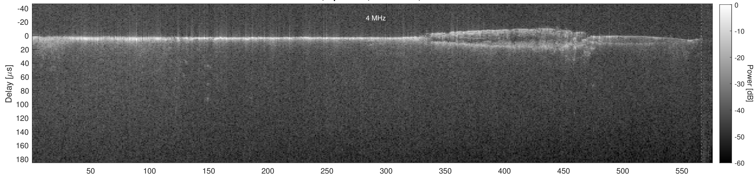
Orbit 5535, Cluttergram
