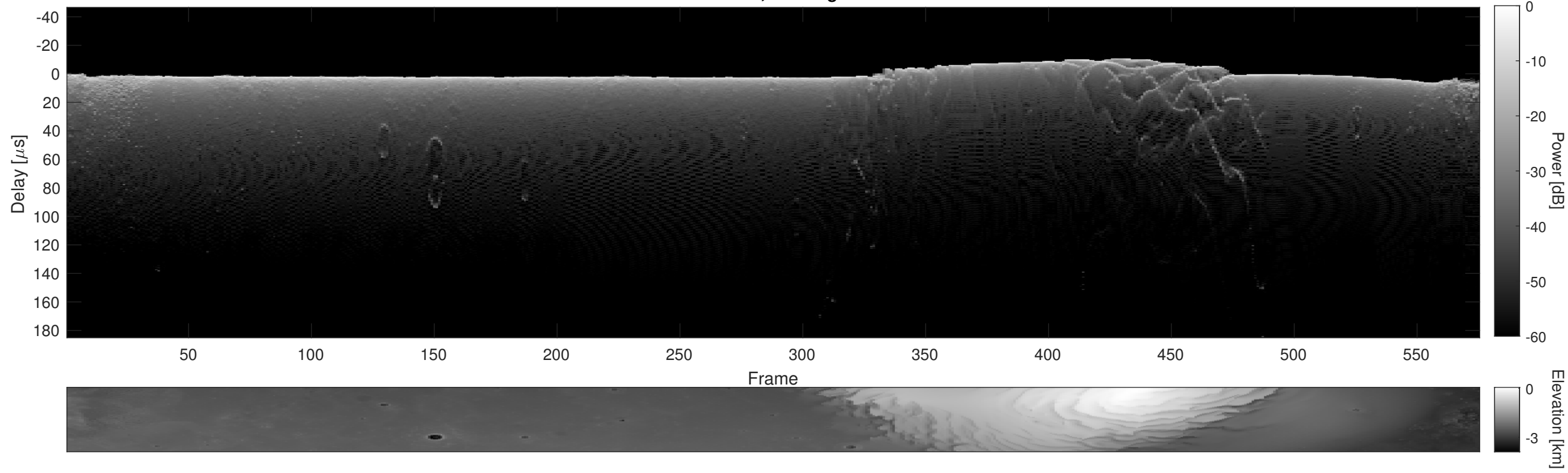
Orbit 5535, Cluttergram
