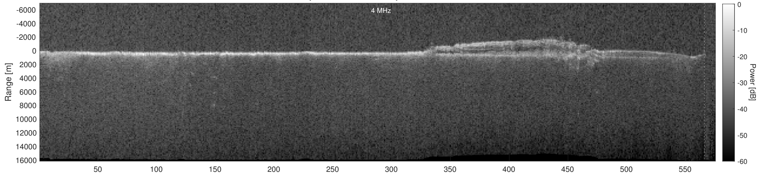
Orbit 5535, Depth-Corrected Cluttergram
