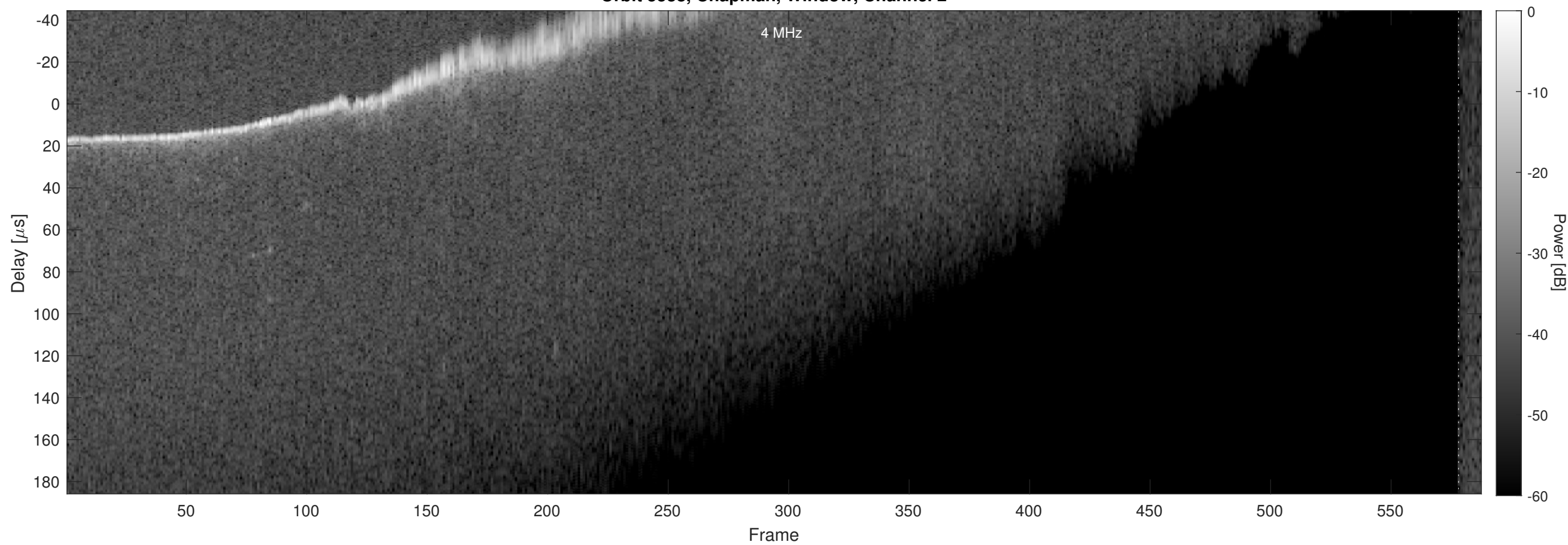
Orbit 5538, Chapman, Window, Channel 2
