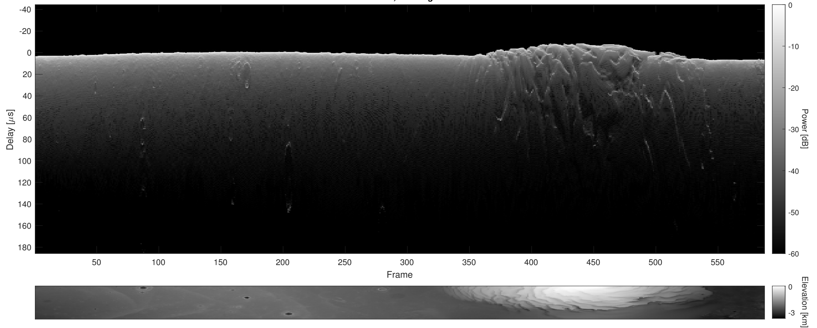
Orbit 5538, Cluttergram
