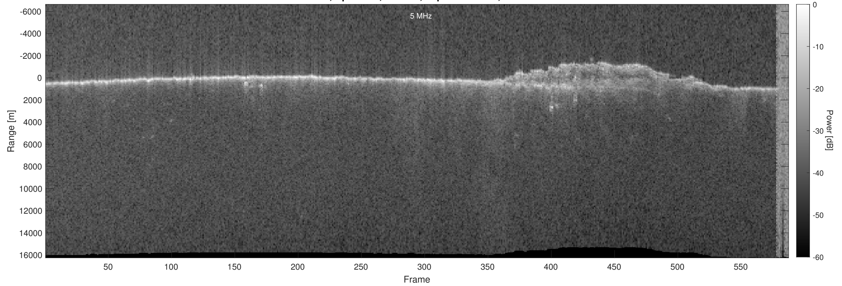
Orbit 5538, Optimized, Window, Depth-Corrected, Channel 2
