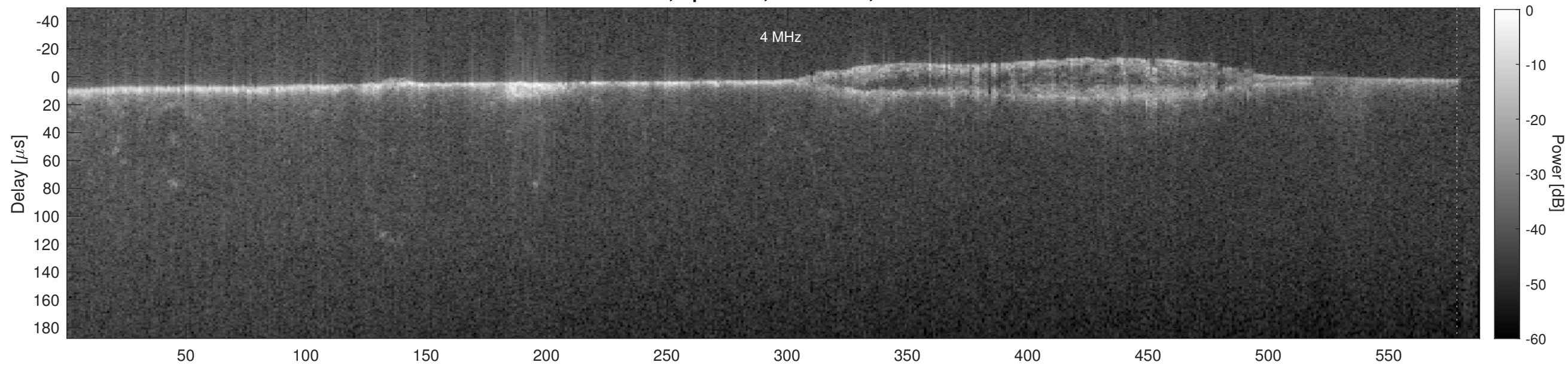
Orbit 5539, Cluttergram
