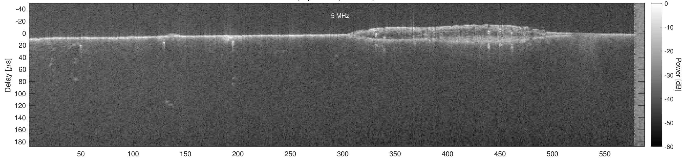
Orbit 5539, Optimized, Window, Channel 2
