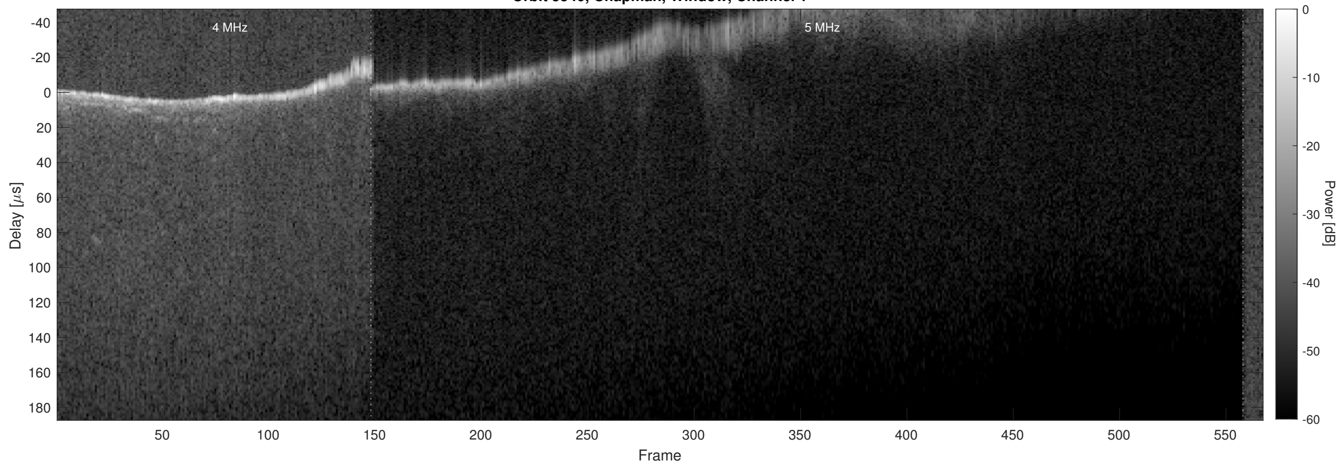
Orbit 5540, Chapman, Window, Channel 2
