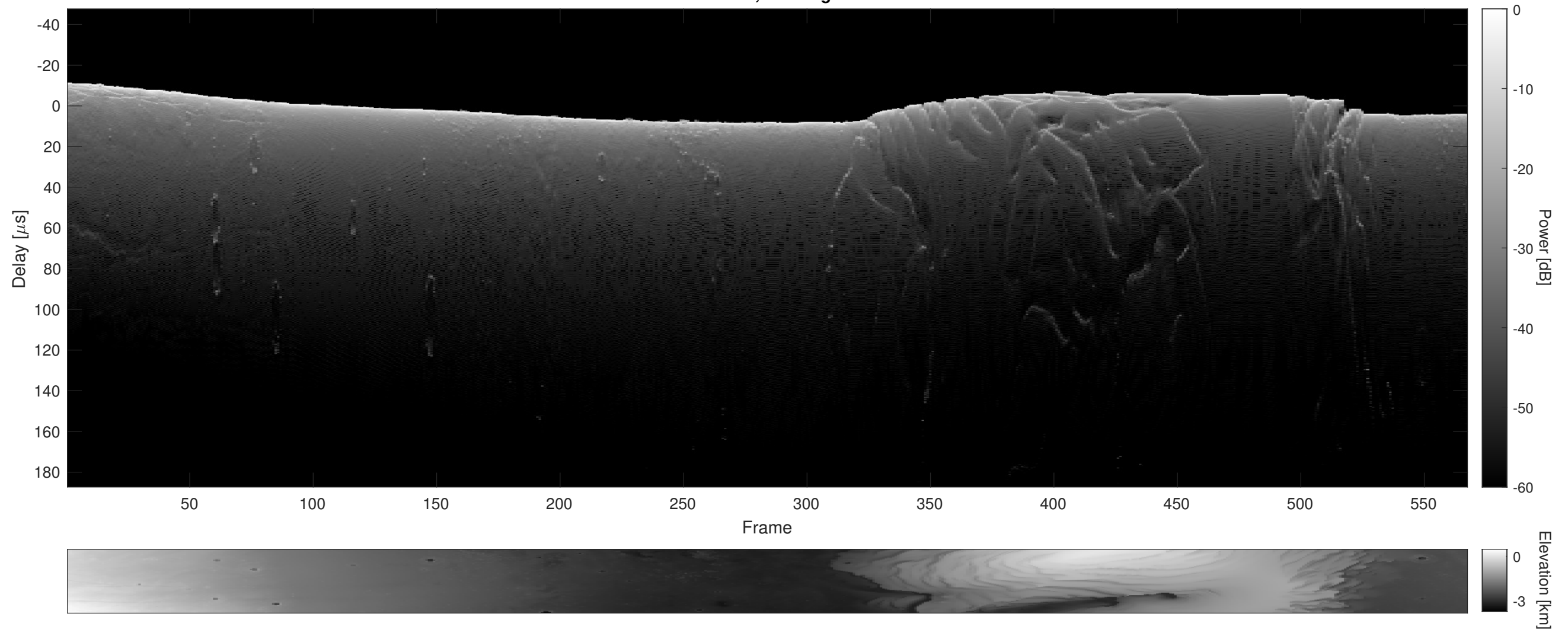
Orbit 5540, Cluttergram
