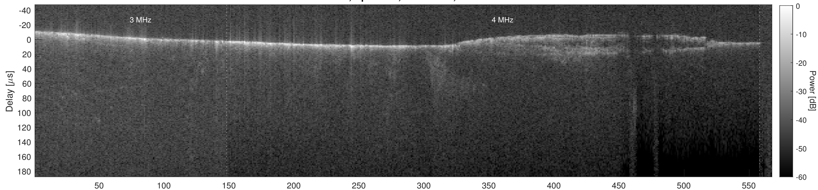
Orbit 5540, Cluttergram
