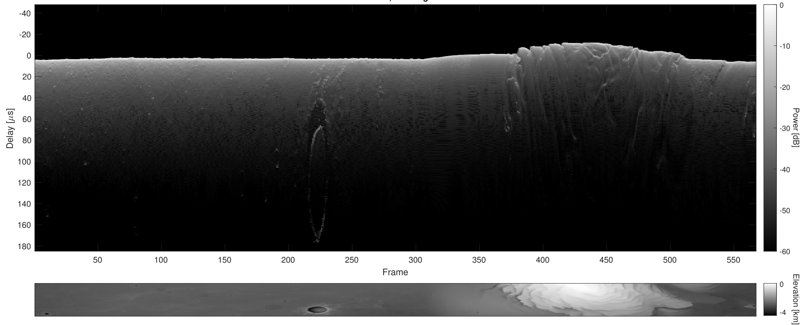
Orbit 5541, Cluttergram
