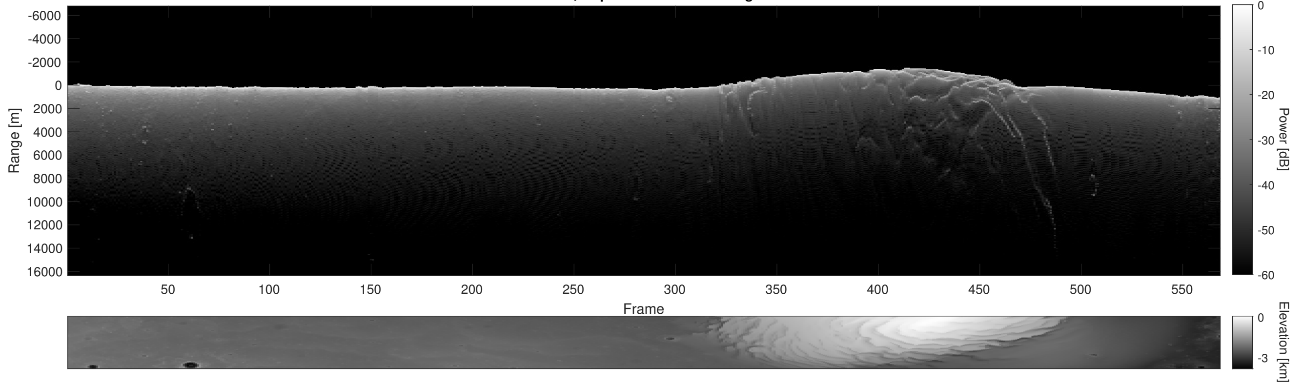
Orbit 5542, Depth-Corrected Cluttergram
