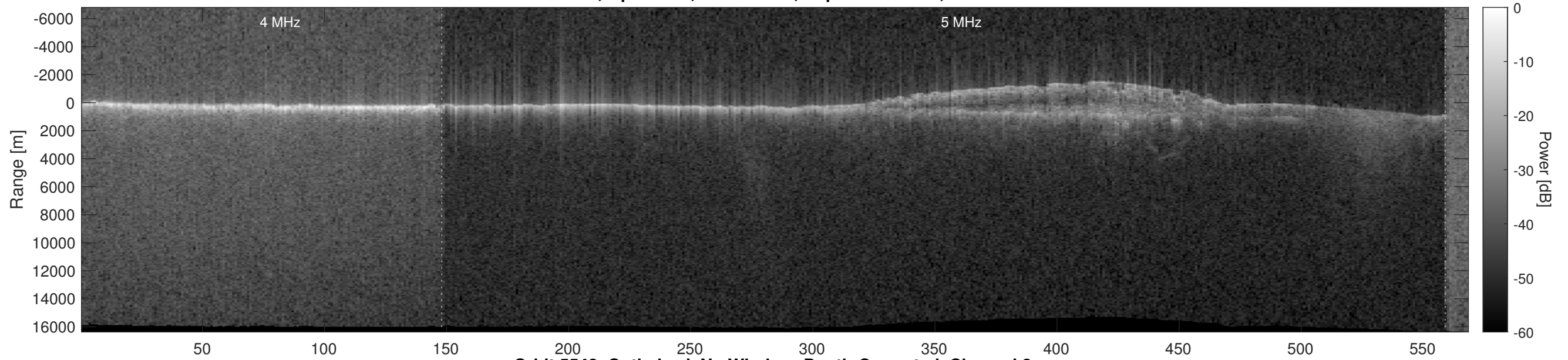
Orbit 5542, Optimized, No Window, Depth-Corrected, Channel 2
