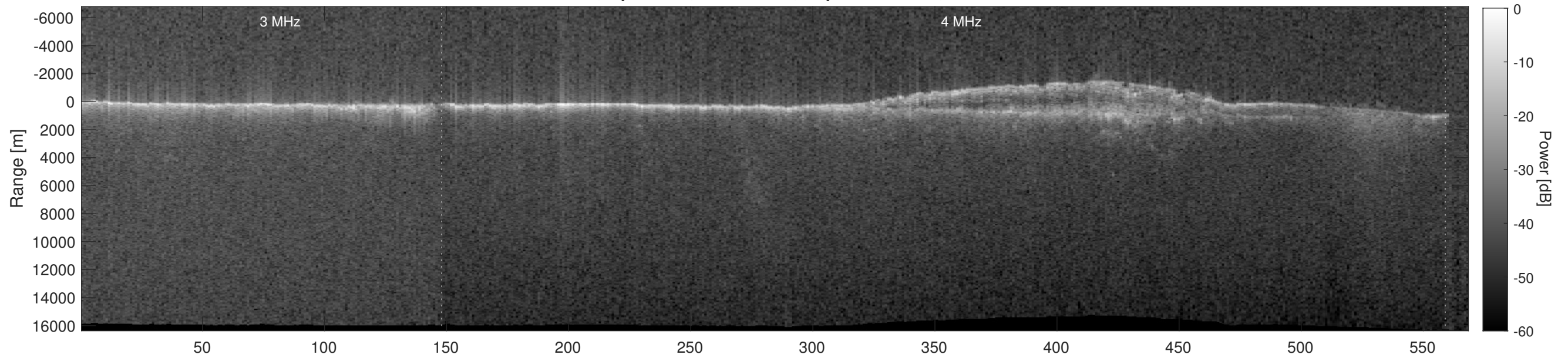
Orbit 5542, Depth-Corrected Cluttergram
