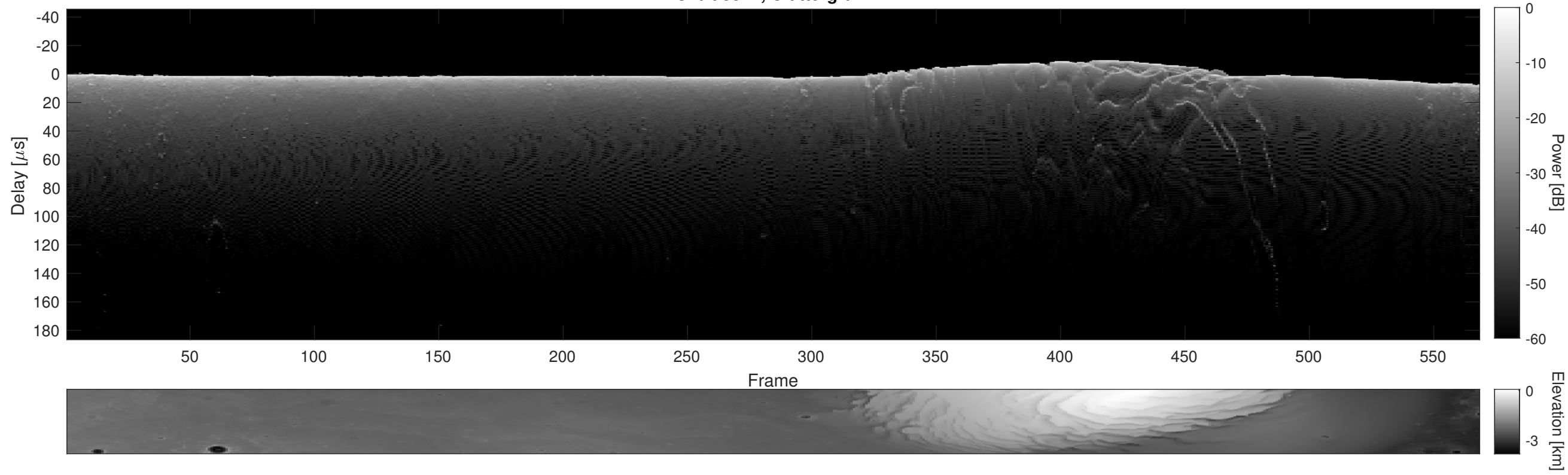
Orbit 5542, Cluttergram
