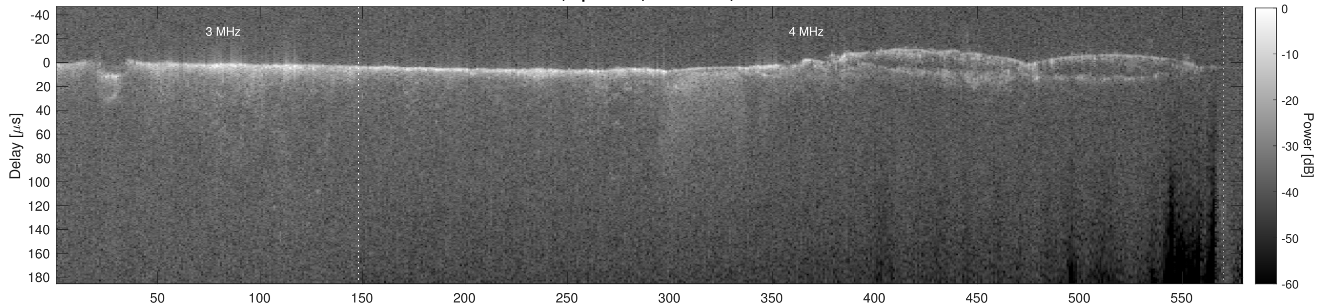
Orbit 5544, Cluttergram
