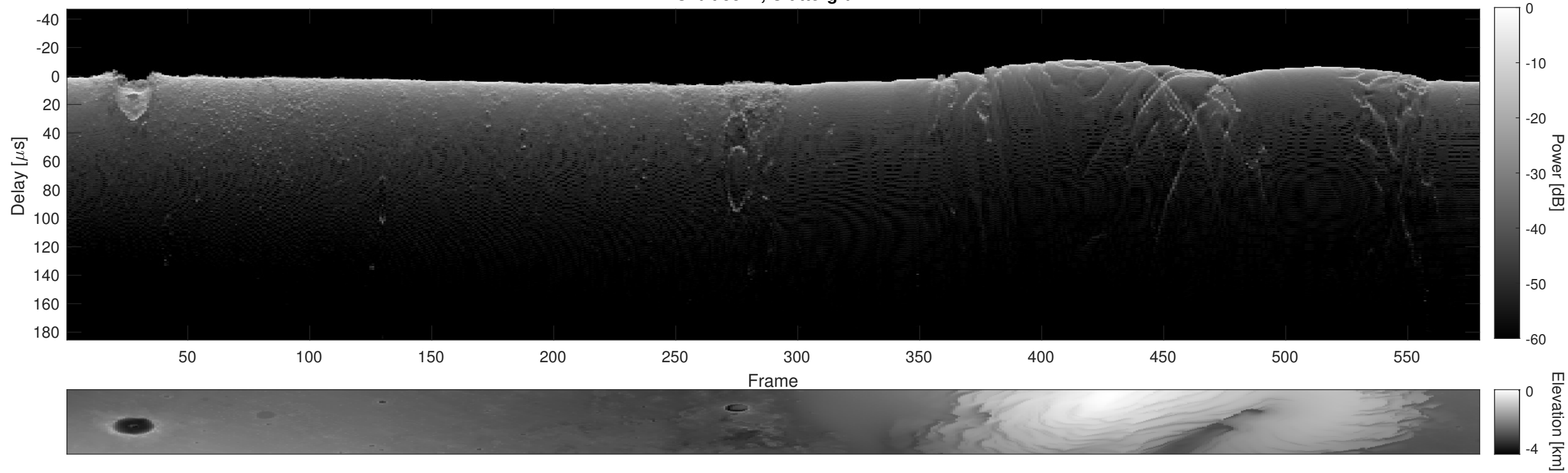
Orbit 5544, Cluttergram
