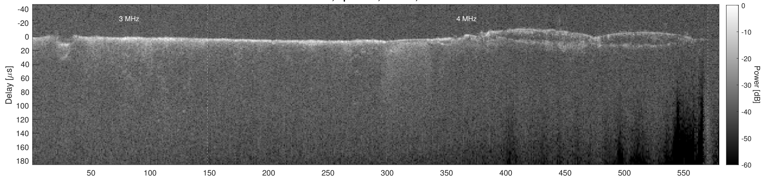
Orbit 5544, Cluttergram
