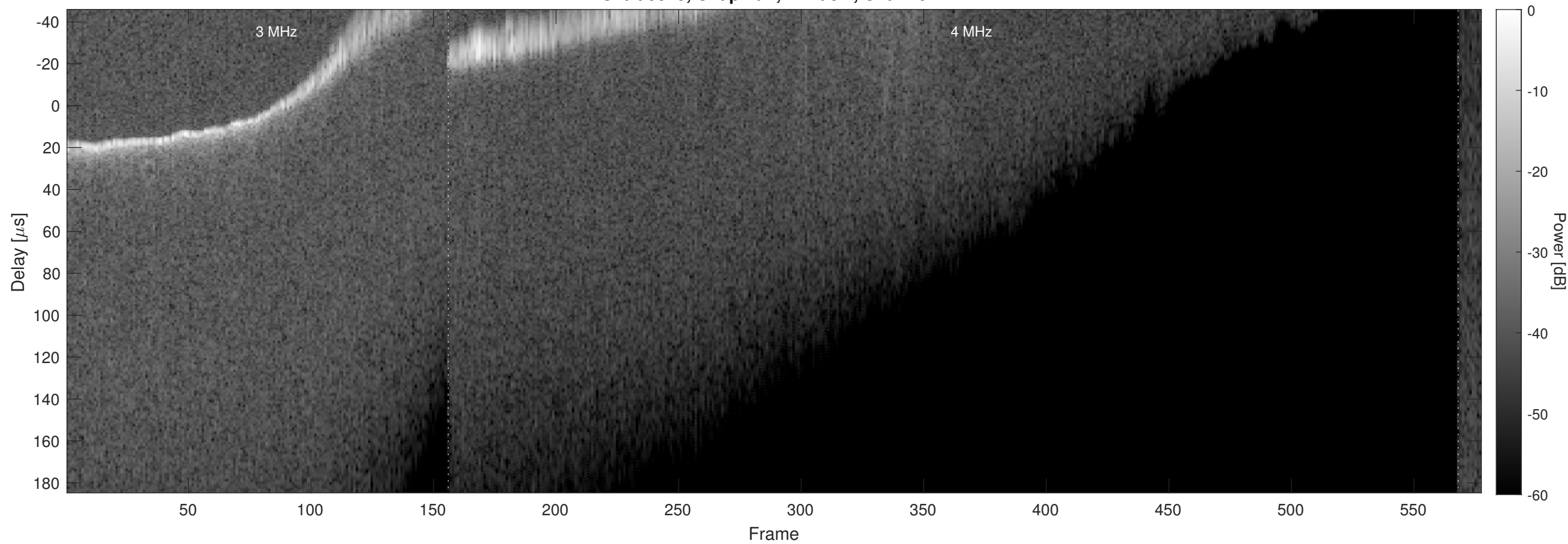
Orbit 5545, Chapman, Window, Channel 2
