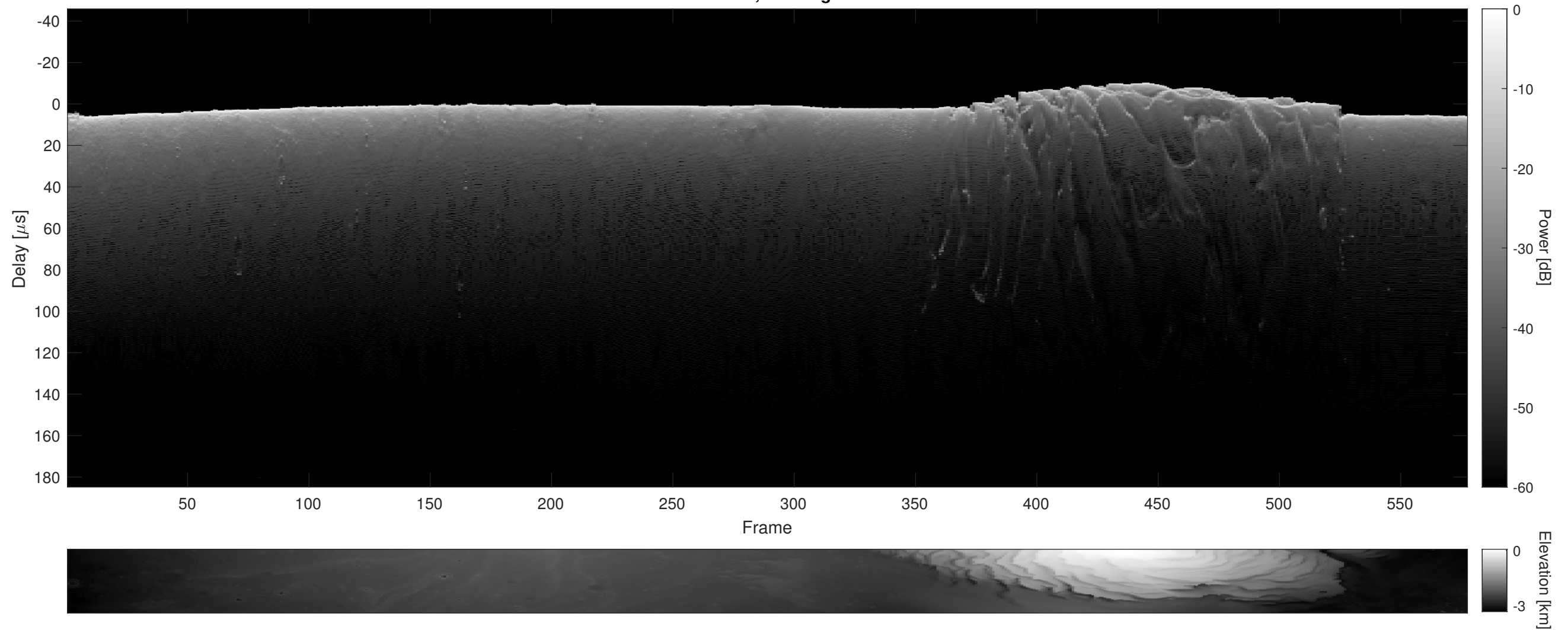
Orbit 5545, Cluttergram
