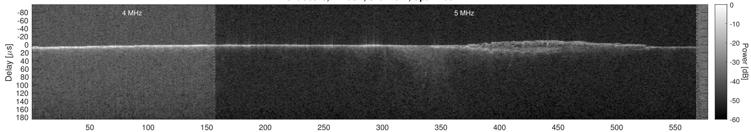
Orbit 5545, Cluttergram
