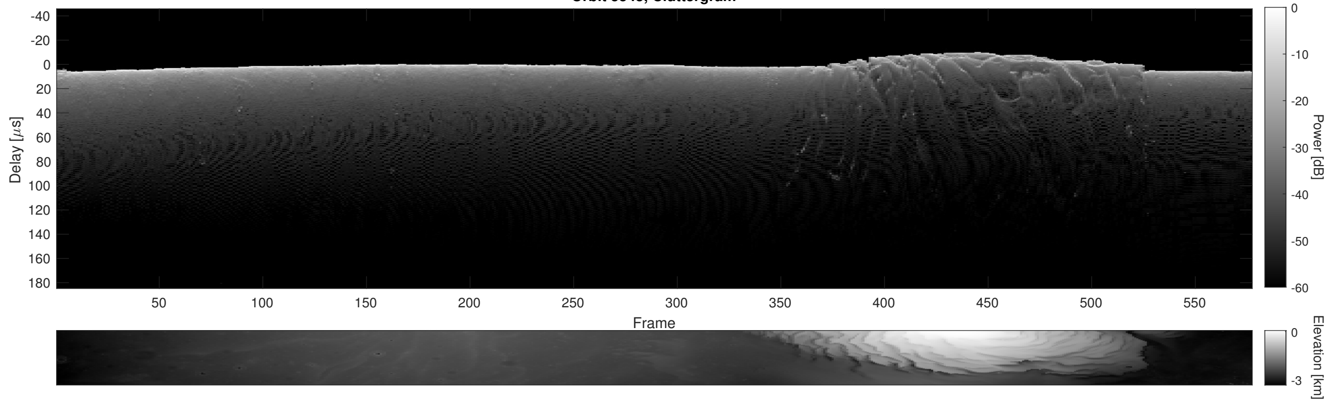
Orbit 5545, Cluttergram
