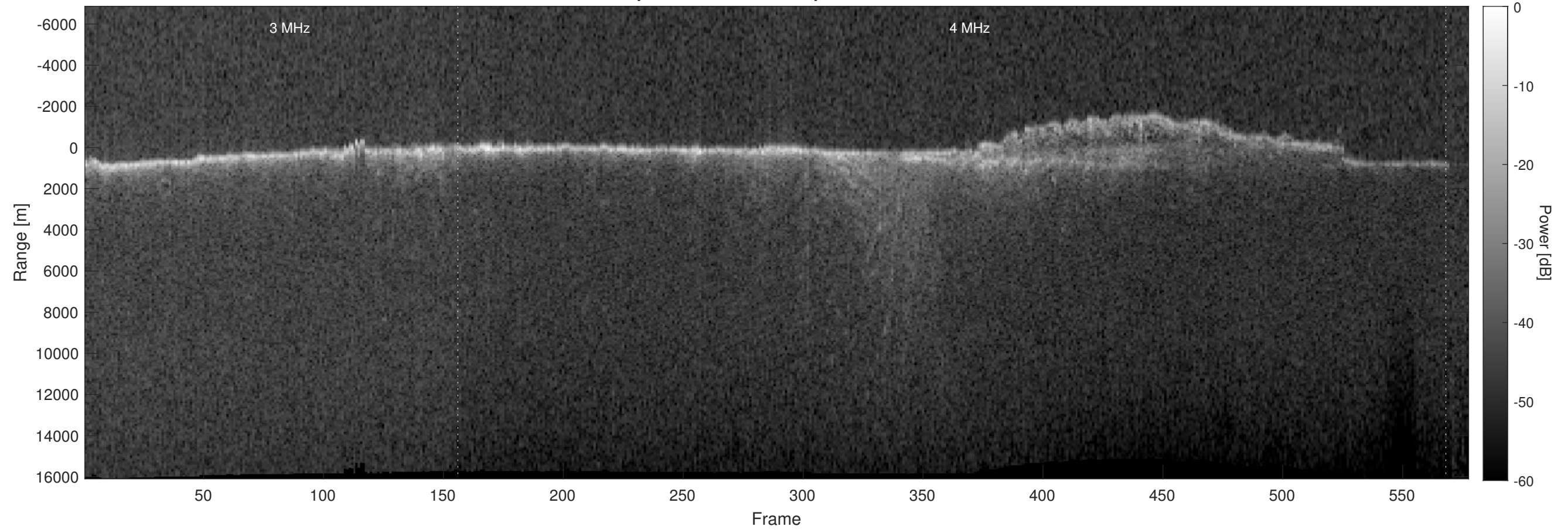
Orbit 5545, Optimized, Window, Depth-Corrected, Channel 2
