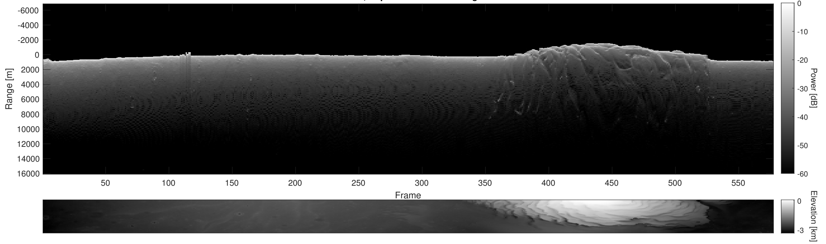
Orbit 5545, Depth-Corrected Cluttergram
