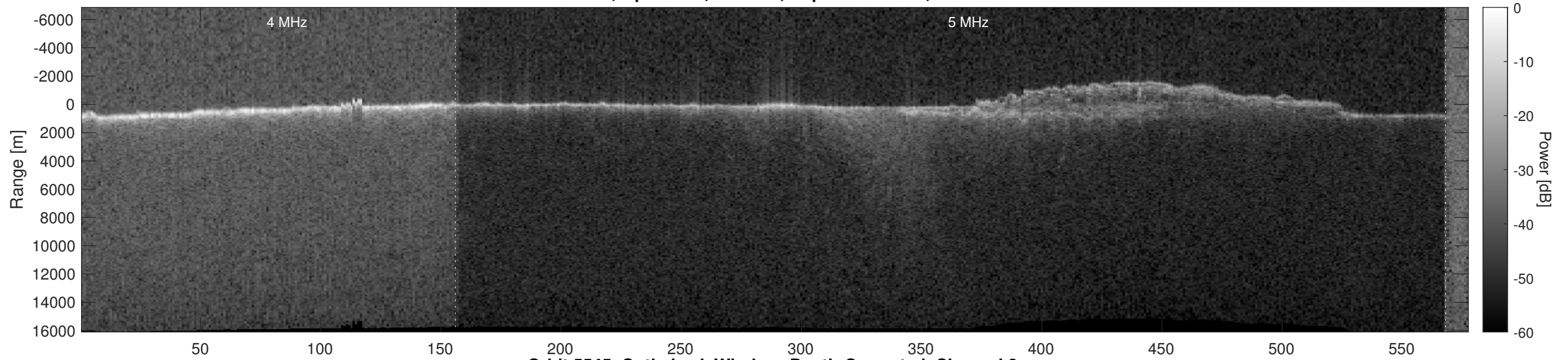
Orbit 5545, Optimized, Window, Depth-Corrected, Channel 2
