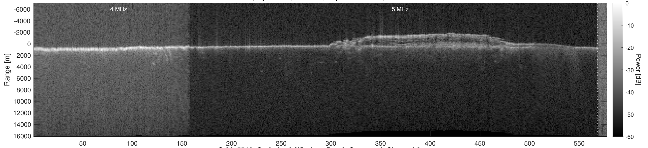
Orbit 5546, Optimized, Window, Depth-Corrected, Channel 2
