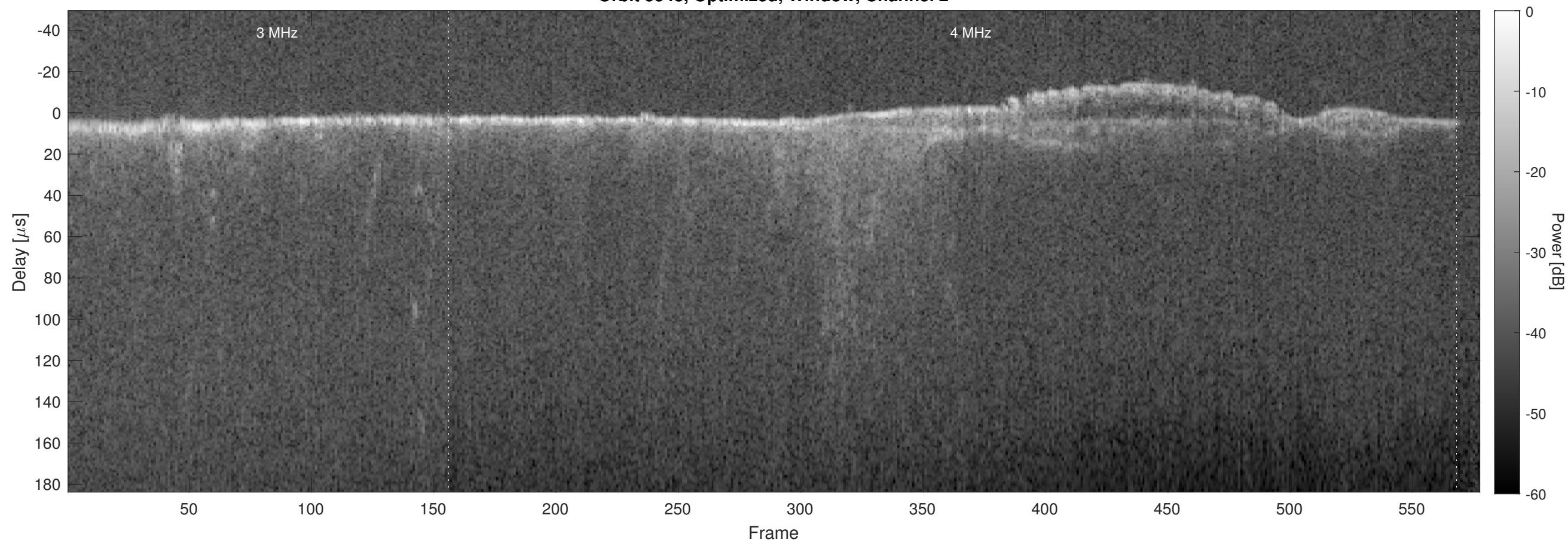
Orbit 5548, Optimized, Window, Channel 2
