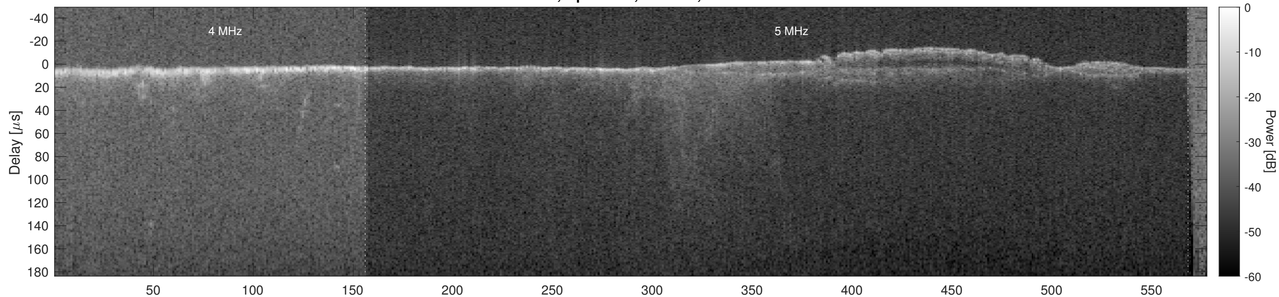
Orbit 5548, Optimized, Window, Channel 2
