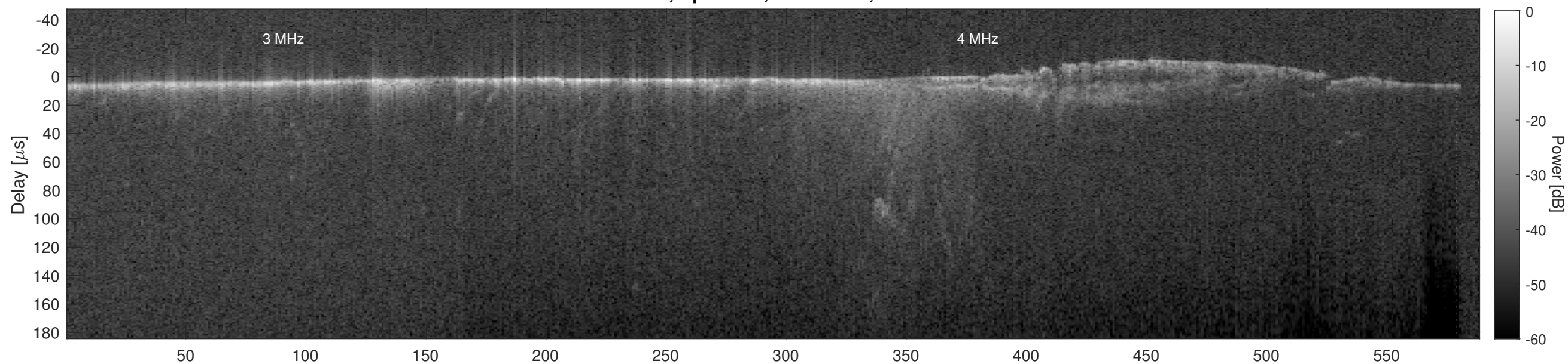
Orbit 5552, Cluttergram
