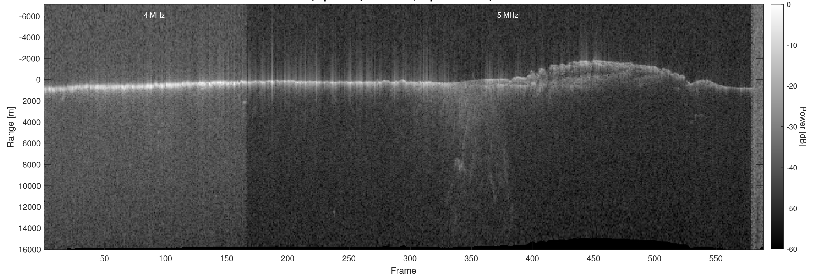
Orbit 5552, Optimized, No Window, Depth-Corrected, Channel 2
