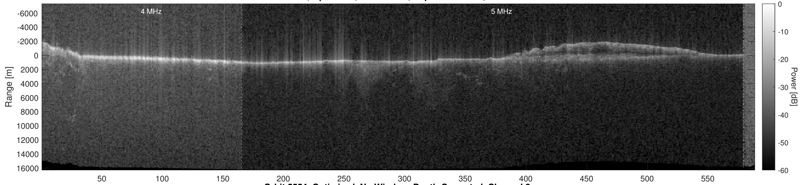
Orbit 5554, Optimized, No Window, Depth-Corrected, Channel 2
