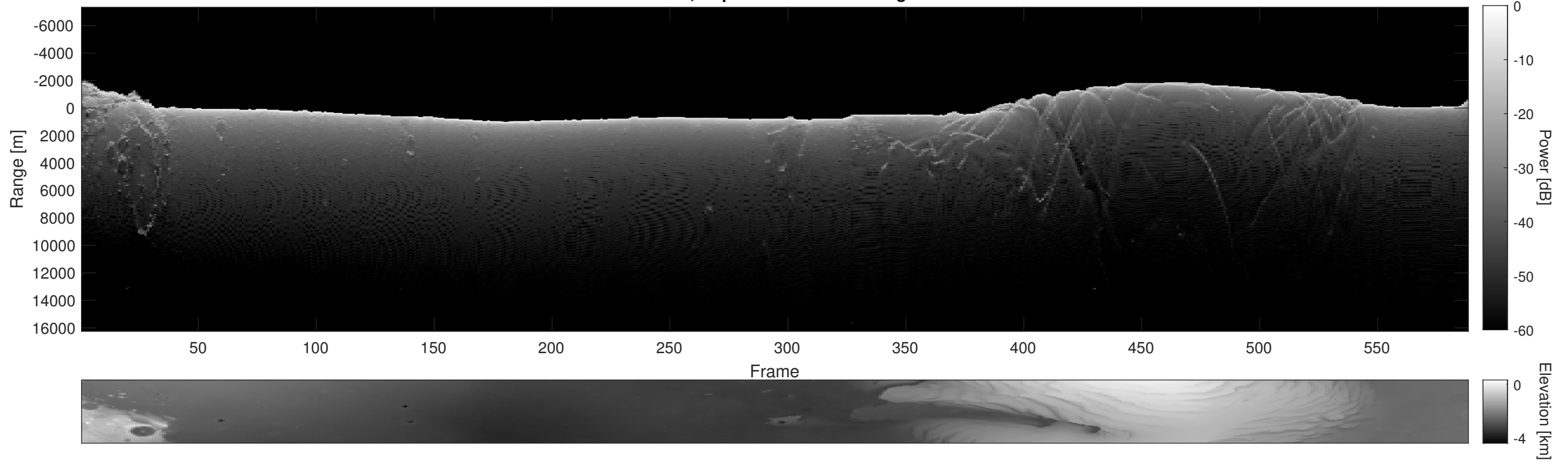
Orbit 5554, Depth-Corrected Cluttergram
