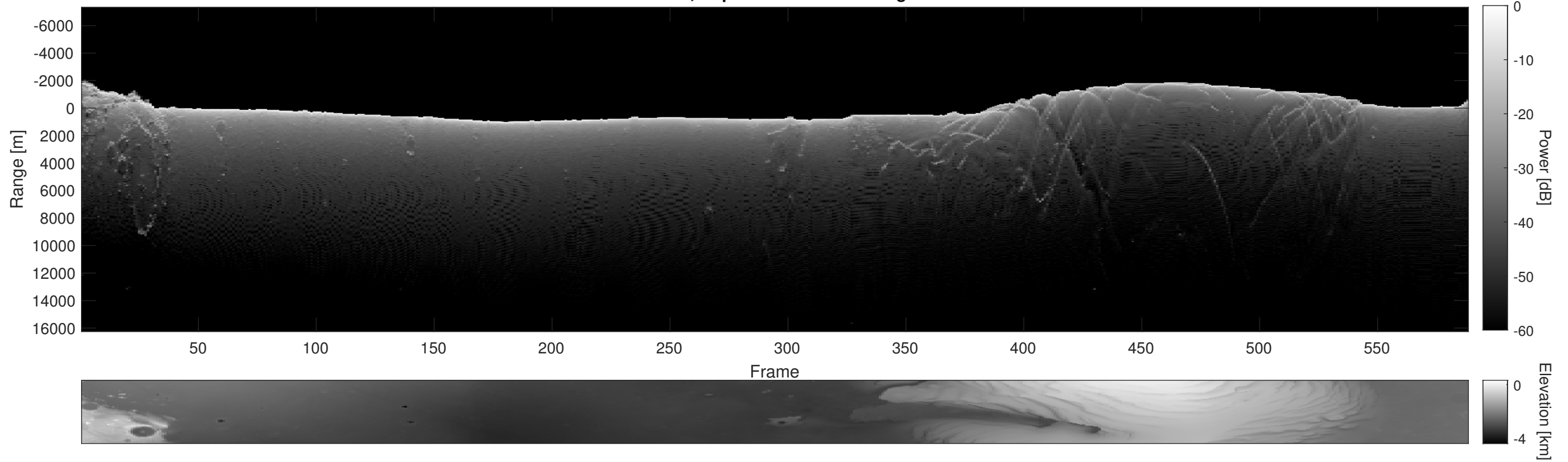
Orbit 5554, Depth-Corrected Cluttergram
