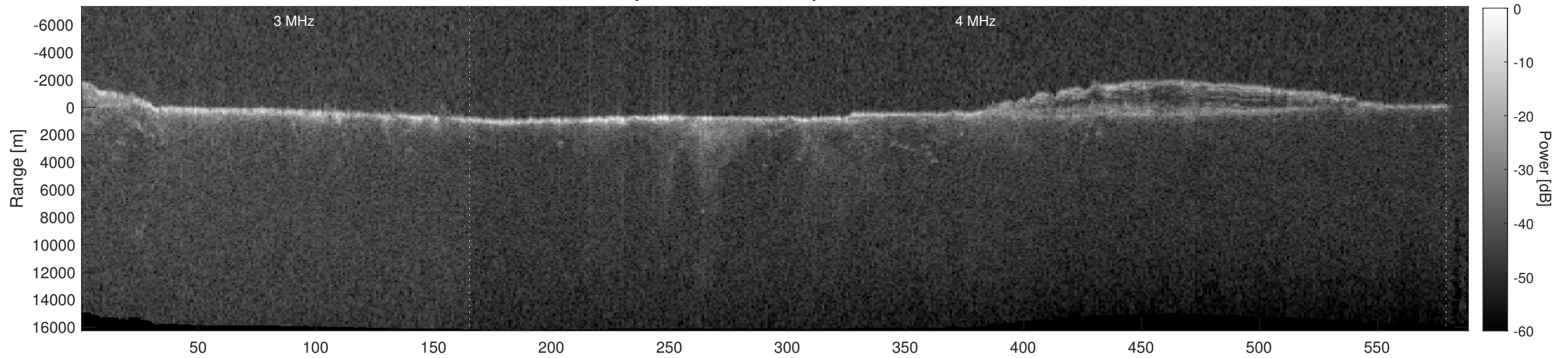
Orbit 5554, Depth-Corrected Cluttergram
