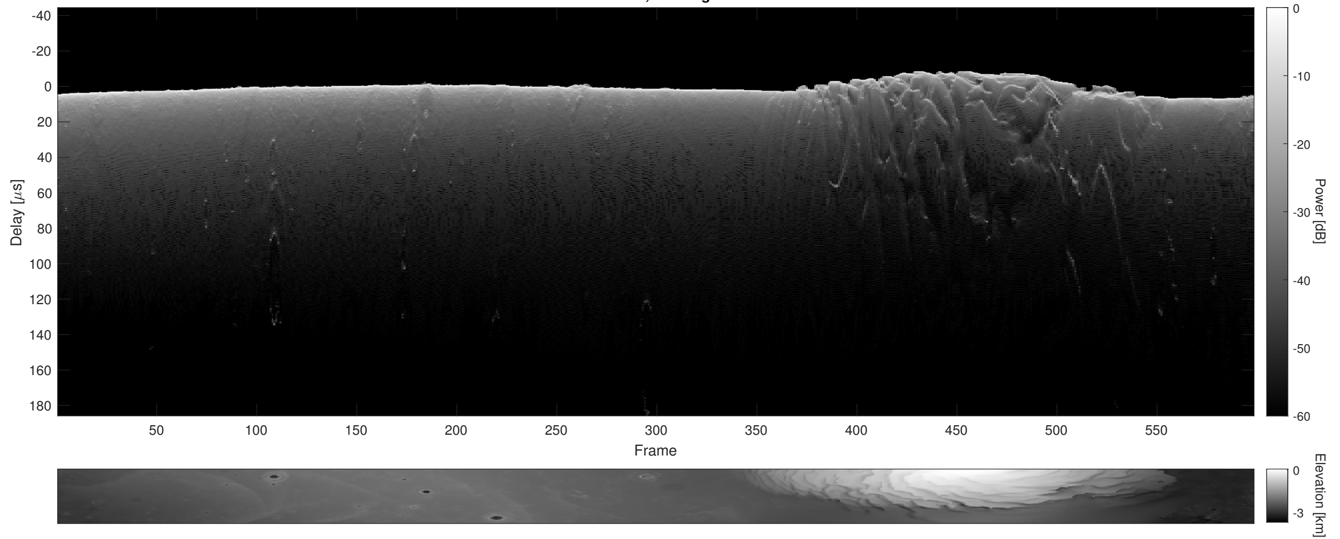
Orbit 5556, Cluttergram
