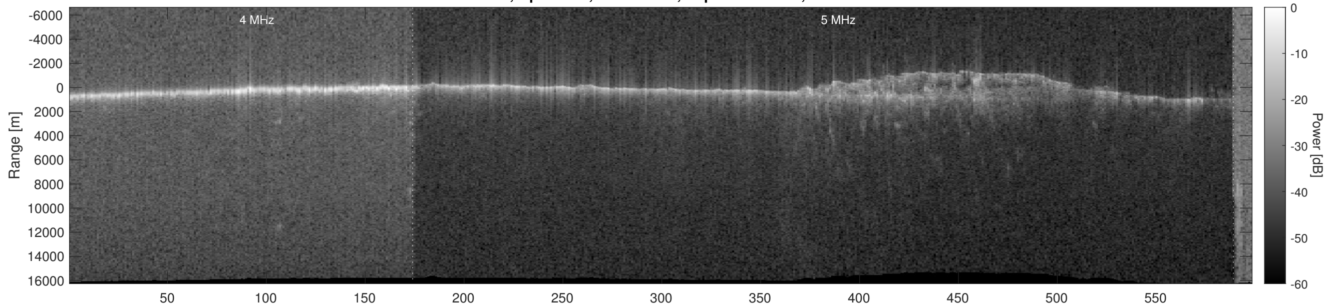
Orbit 5556, Optimized, No Window, Depth-Corrected, Channel 2
