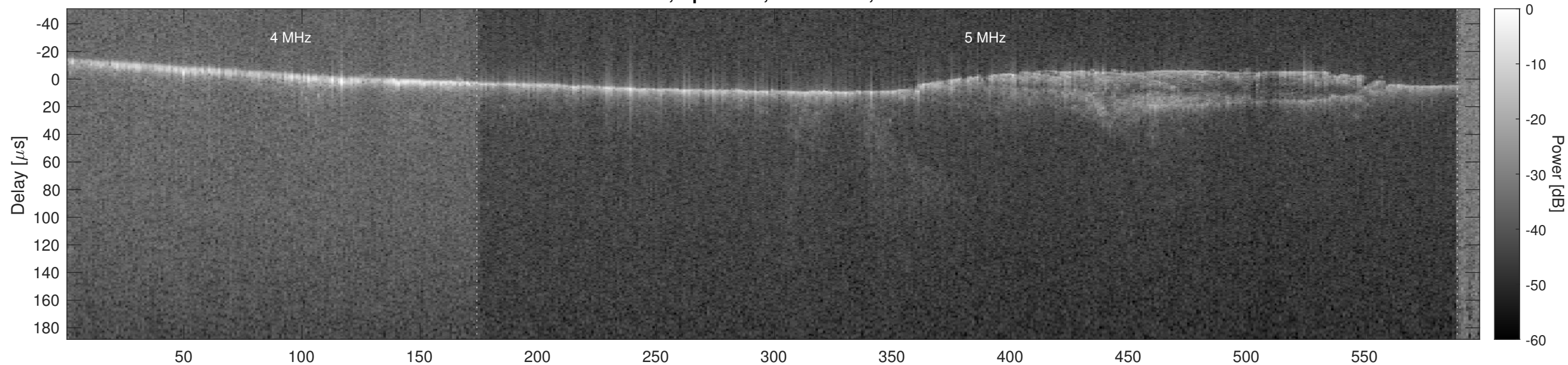
Orbit 5558, Optimized, No Window, Channel 2
