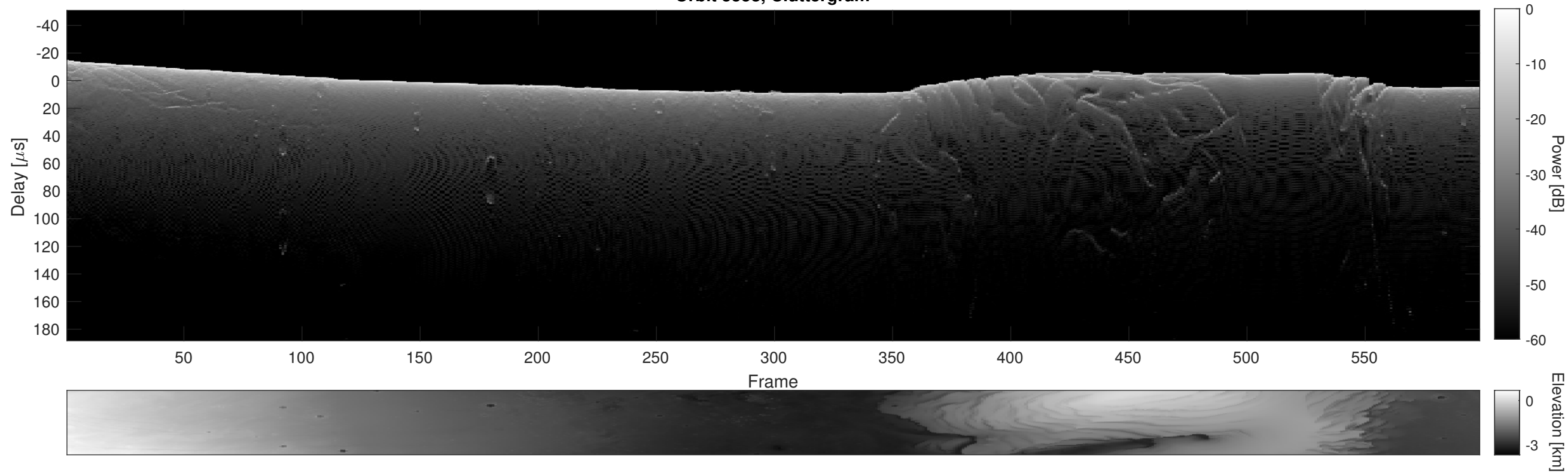
Orbit 5558, Cluttergram
