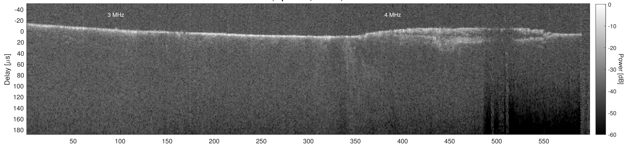
Orbit 5558, Cluttergram
