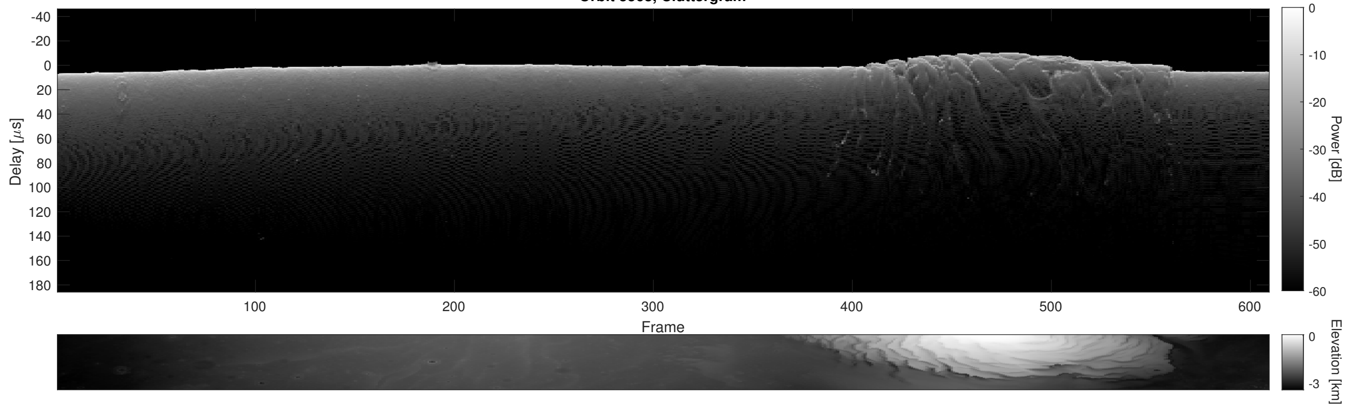
Orbit 5563, Cluttergram
