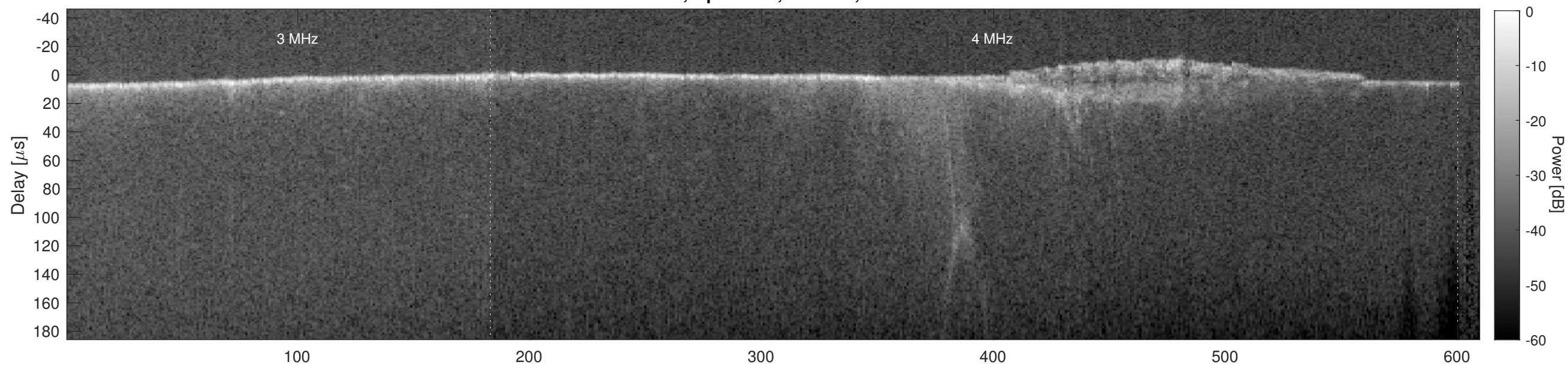
Orbit 5563, Cluttergram
