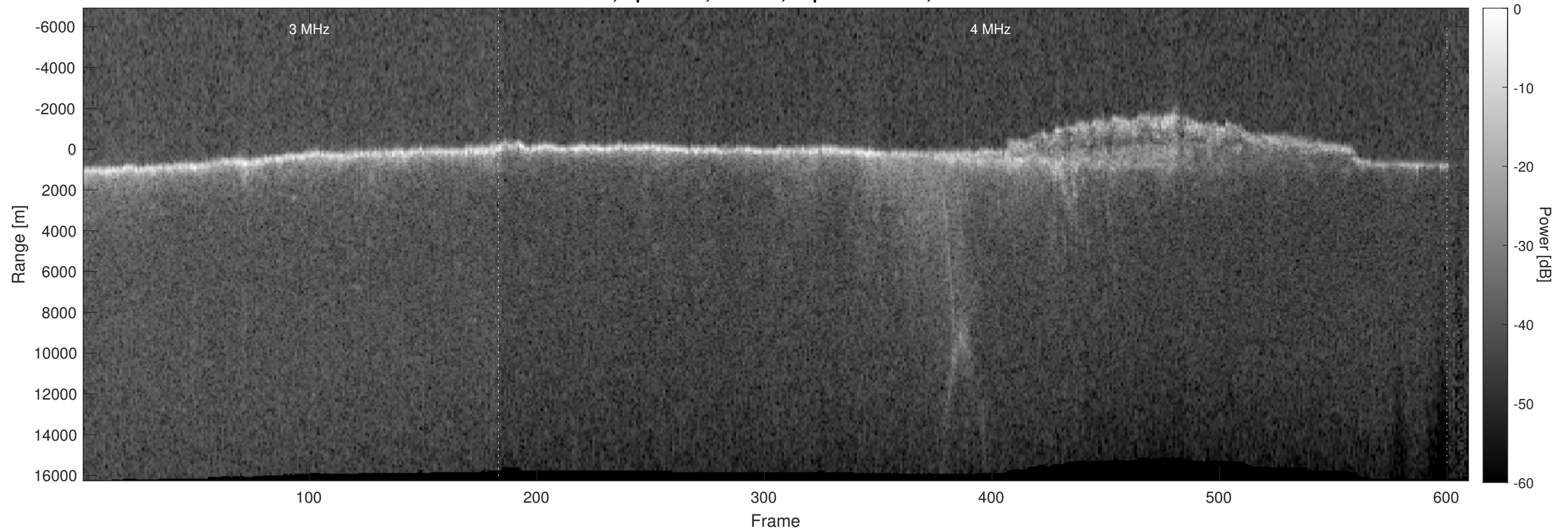
Orbit 5563, Optimized, Window, Depth-Corrected, Channel 2
