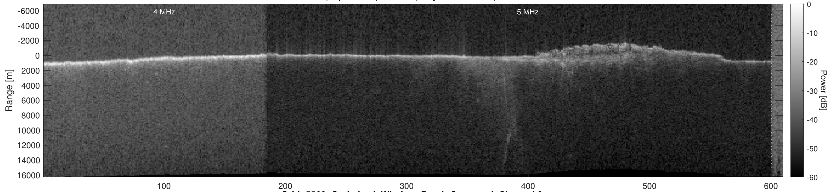
Orbit 5563, Optimized, Window, Depth-Corrected, Channel 2
