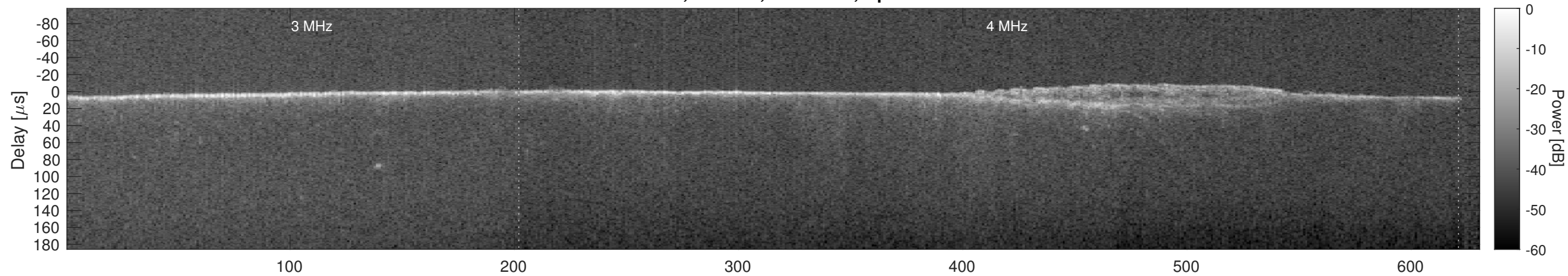
Orbit 5574, Cluttergram
