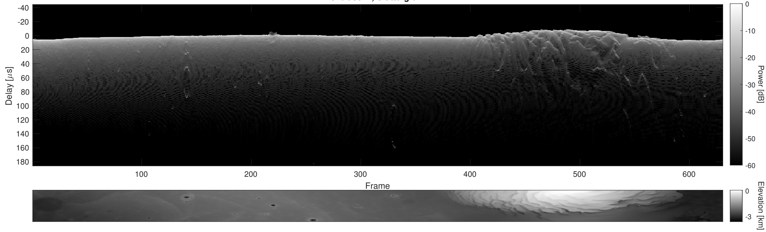
Orbit 5574, Cluttergram
