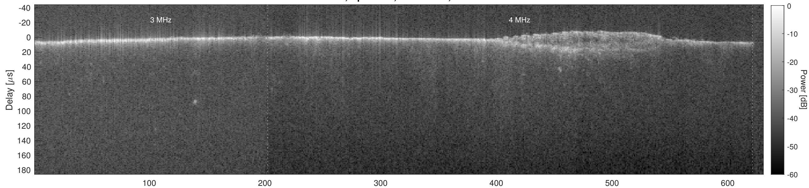
Orbit 5574, Cluttergram
