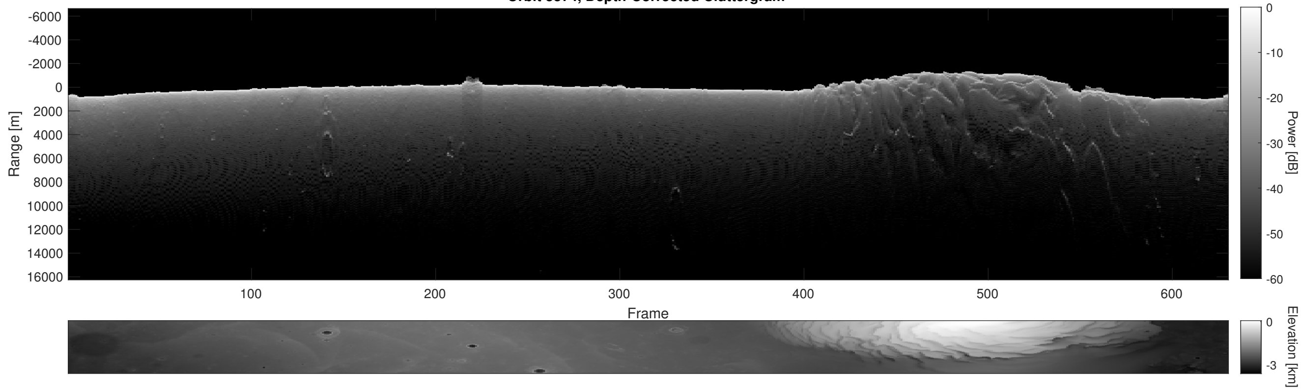
Orbit 5574, Depth-Corrected Cluttergram
