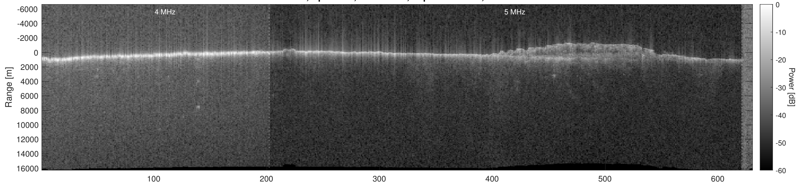
Orbit 5574, Optimized, No Window, Depth-Corrected, Channel 2
