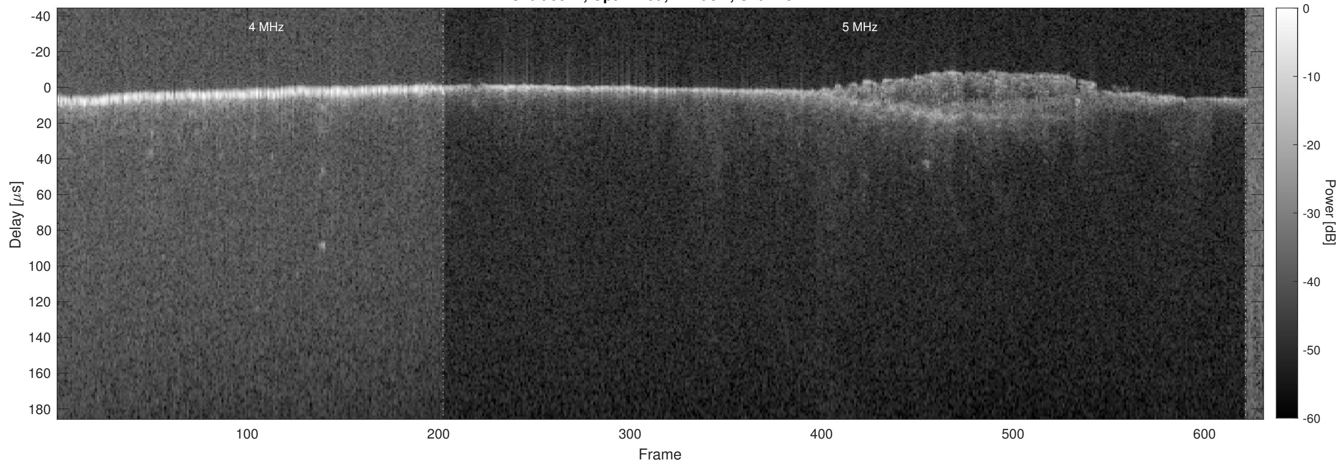
Orbit 5574, Optimized, Window, Channel 2
