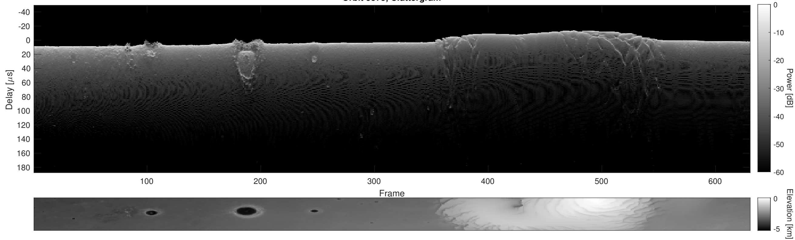
Orbit 5575, Cluttergram
