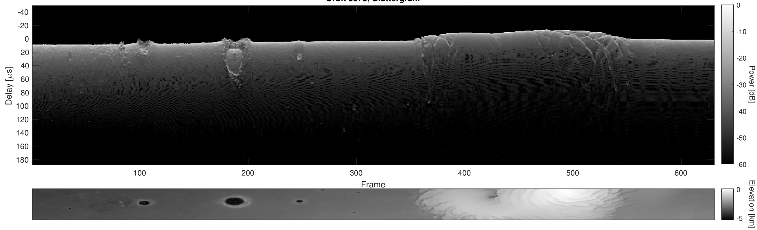
Orbit 5575, Cluttergram
