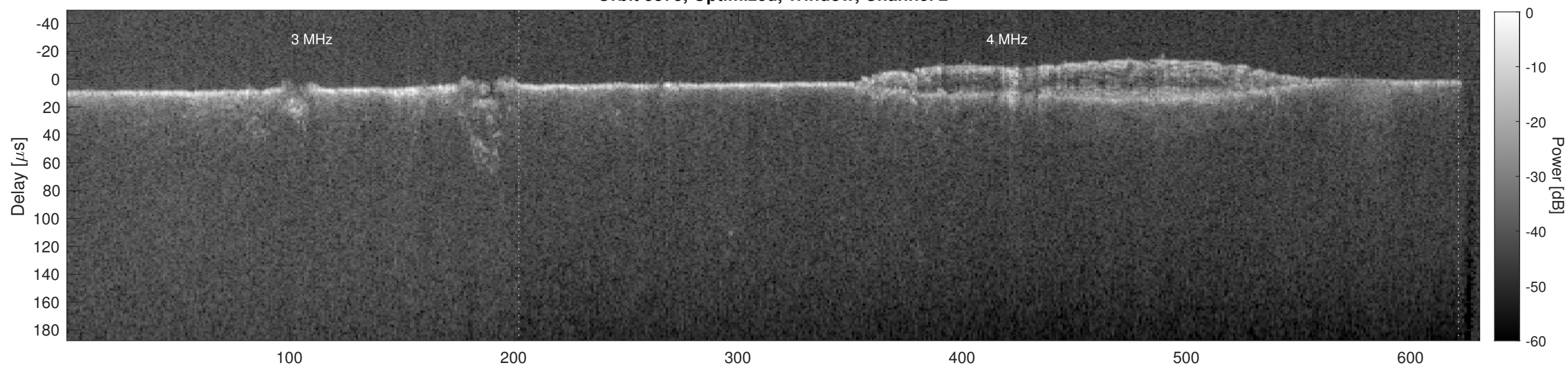
Orbit 5575, Cluttergram
