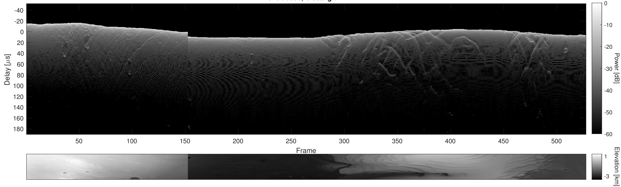
Orbit 5583, Cluttergram
